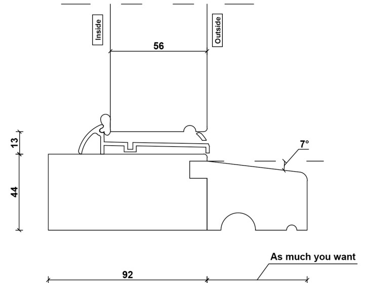
Std ATW 44mm Timber cill + Alu low threshold on top - OPEN OUT
